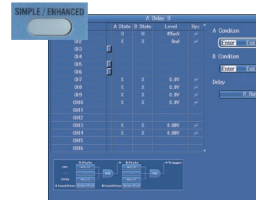
Example: "A delay B" trigger setup screen (After condition A becomes true, trigger the first time condition B becomes true after a set time has passed.)
